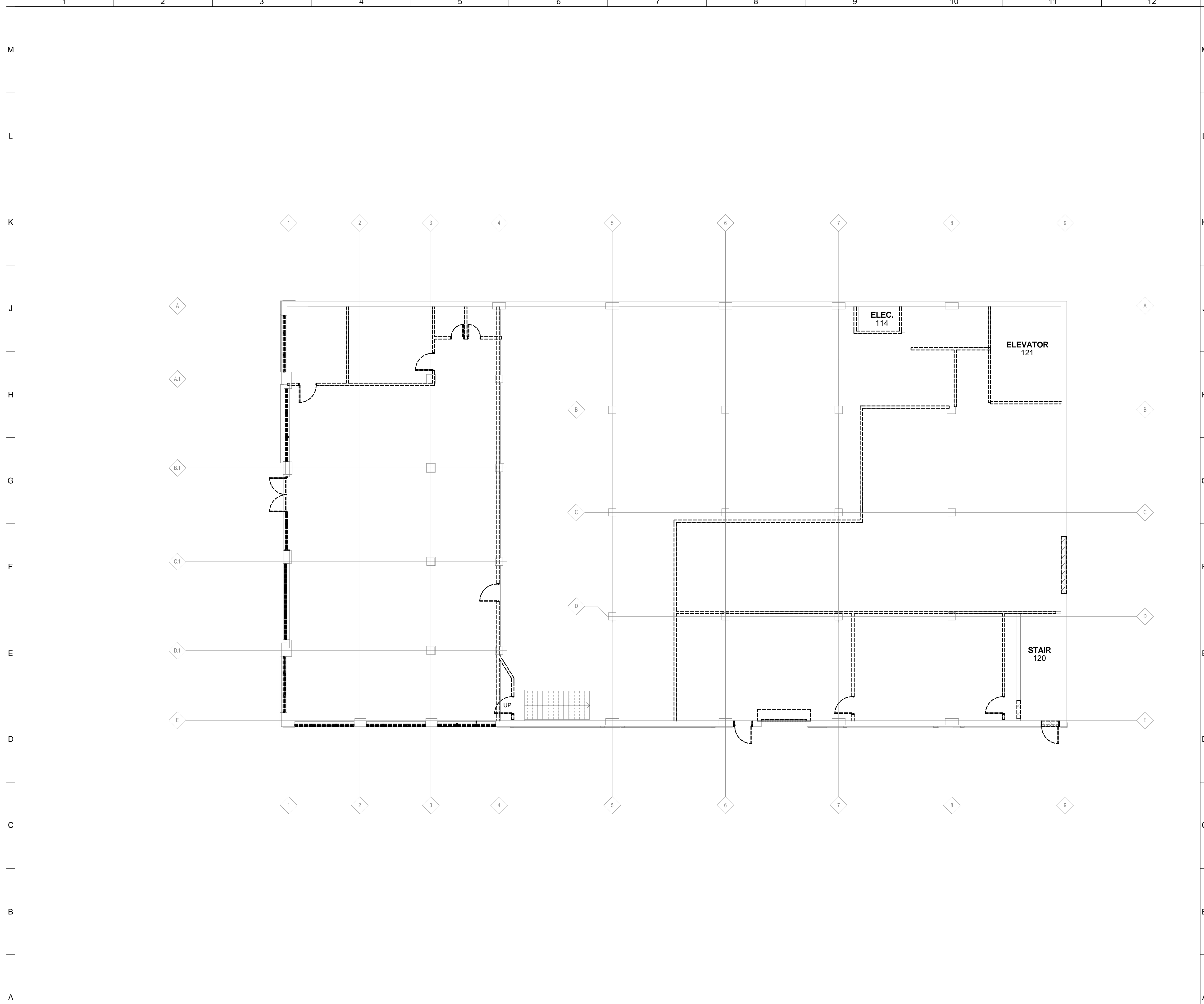
A1 FIRST LEVEL DEMOLITION PLAN SCALE: 1/8" = 1'-0"
